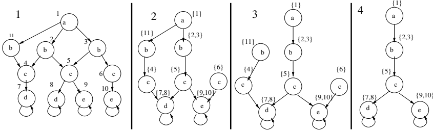
Fig. 4. An example of the Minimizing Algorithm
