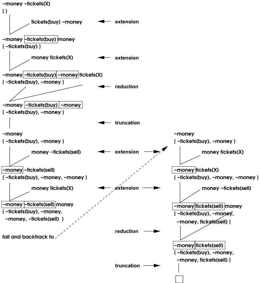
Fig. 1. A PTP+GLiDeS refutation
