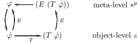
Fig. 1. Schematic overview of the general procedure. The proof of the implication from (E (T \dot{\varphi})) to \varphi can be generated uniformly in \dot{\varphi} .
