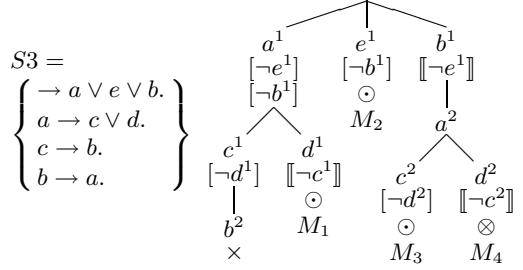
Fig. 7. An MG-tree with branching lemmas
